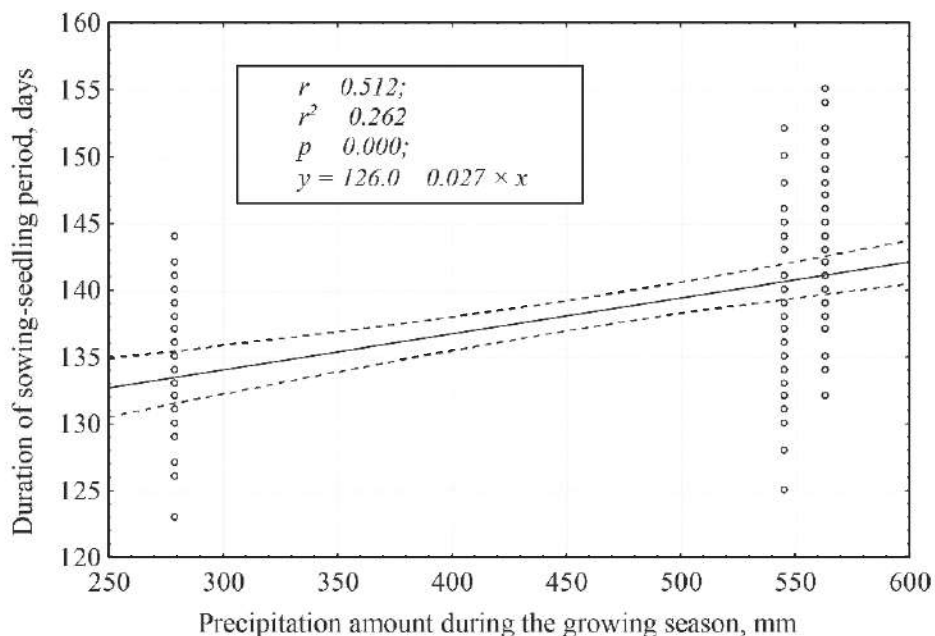
Fig. 2. Correlation relations and the regression equation between precipitation amount during the growing season and its duration
