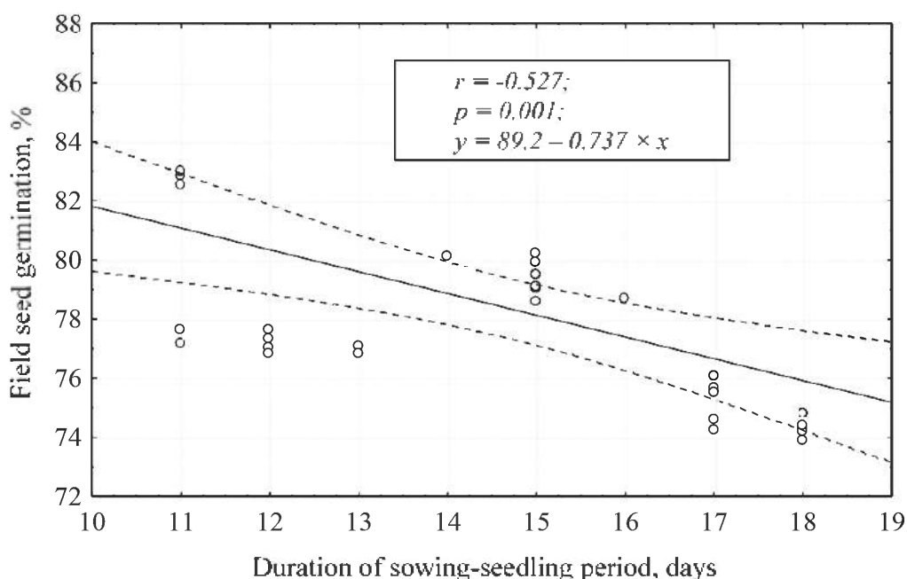
Fig. 1. Correlation relations and regression equations between the duration of sowing-seedling period and the field seed germination of grain sorghum and soriz
